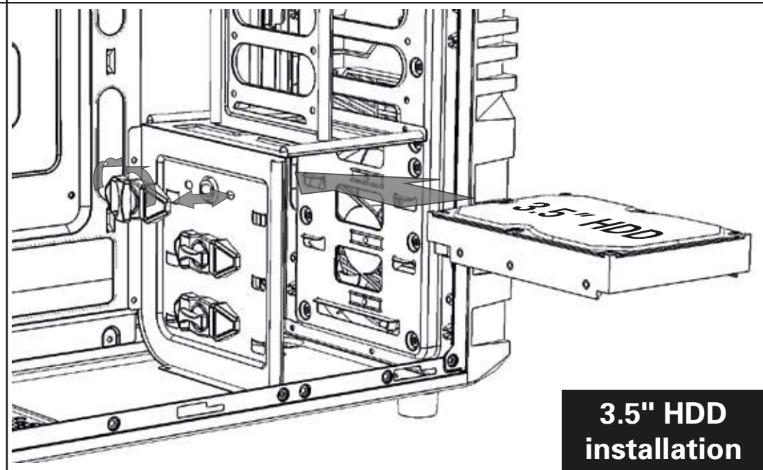
3.5" device installation
