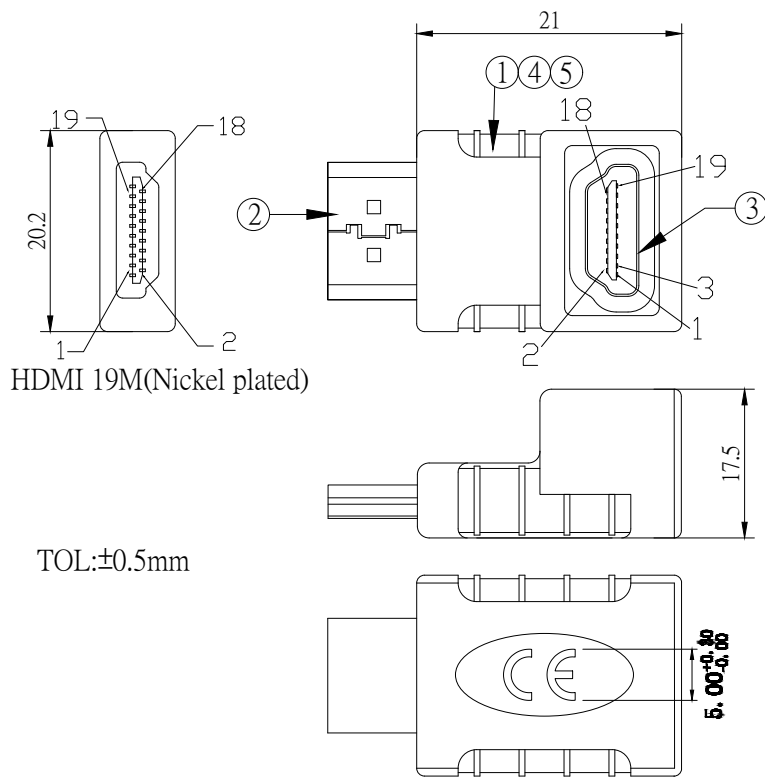
HDMI 19M TO HDMI 19F ADAPTER Black molding
