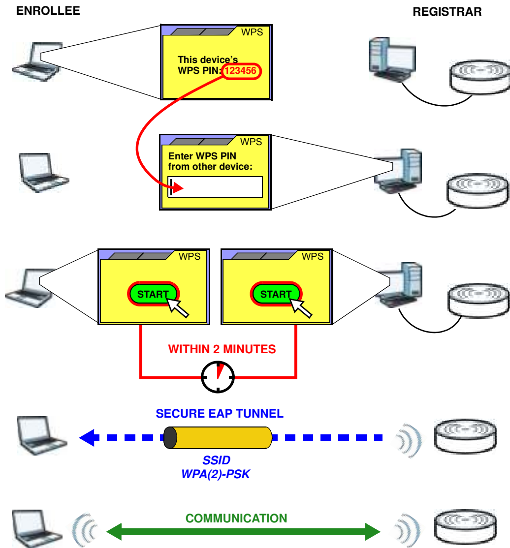
Figure 21 Example WPS Process: PIN Method
