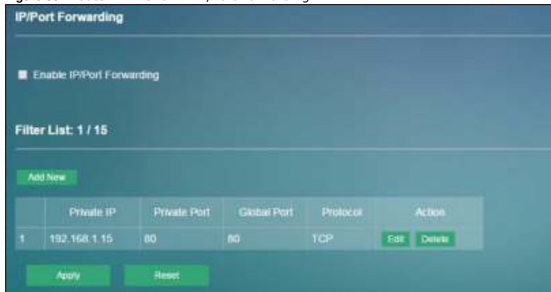
Figure 33 Router > Firewall > IP/Port Forwarding
