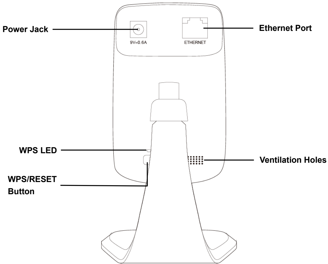
Figure 2-2 Rear Panel
