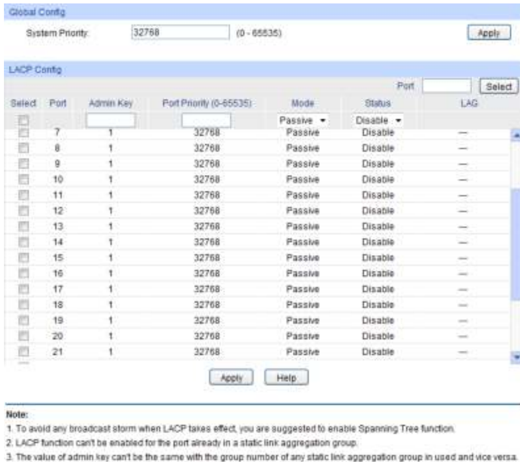
Figure 5-10 LACP Config
