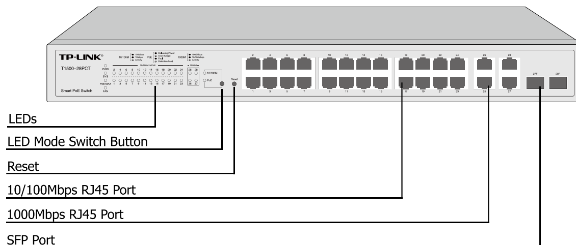
Figure 2-1 Front Panel of T1500-28PCT
